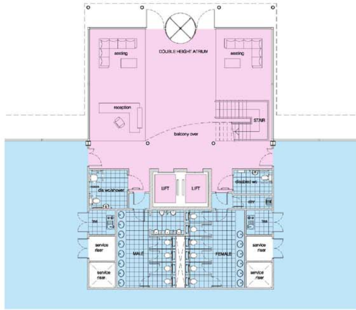
Ground floor main service core
