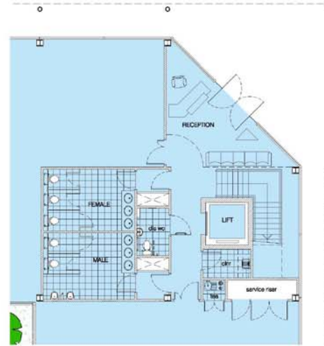
Ground floor secondary service core
